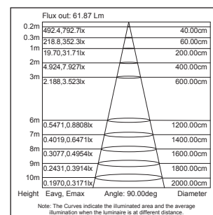
Lux Distance Curve
